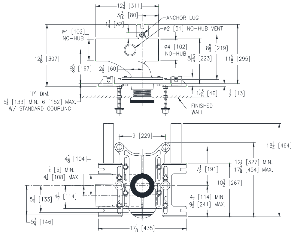
Z1201-NR4-RYK Illustrated
